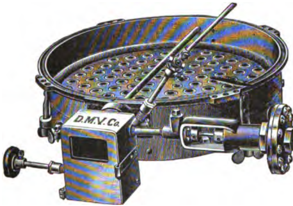
FIG. 212.—The Dayton Burner, showing the Starter Box and Regulator in Position.
